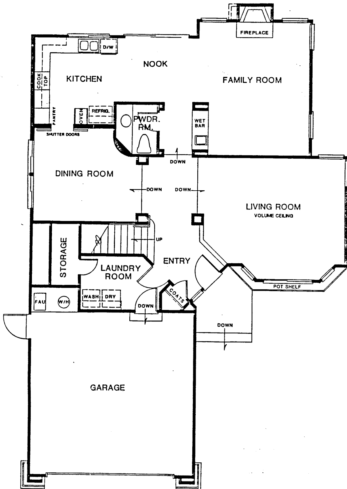
Plan 2—Willow 2338 square feet
